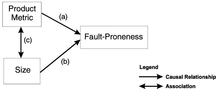
Fig. 2. Path diagram illustrating the confounding effect of size.
