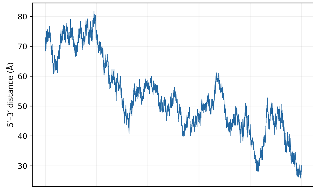
poly(dT)40 structural evolution in 3 M KCl
