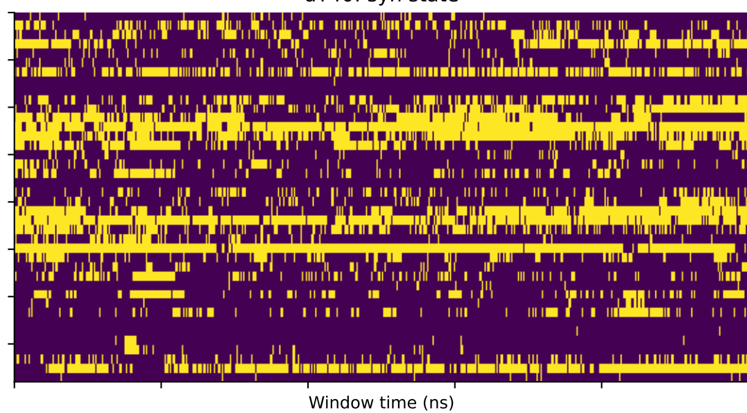
dT40: unstacked from sequence neighbors
