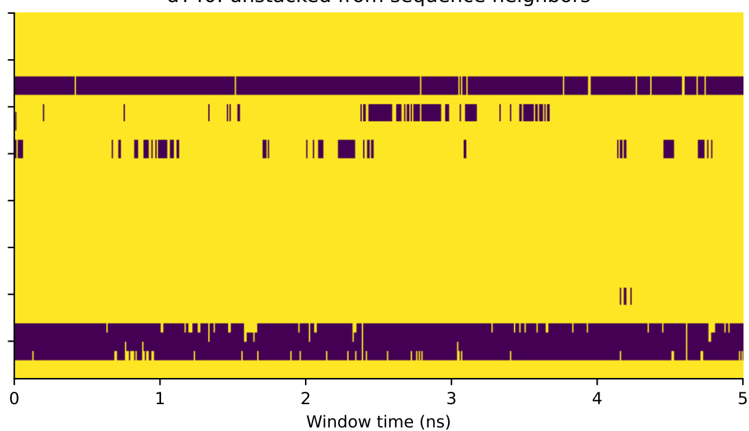
dT40: unstacked from sequence neighbors
