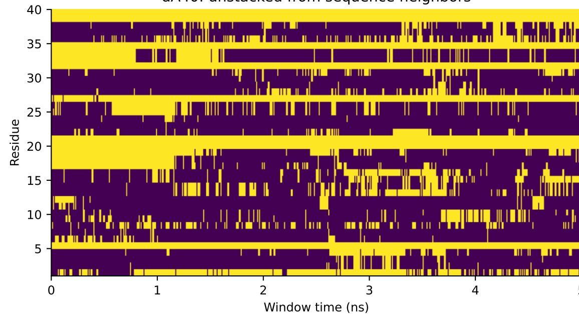
dA40: unstacked from sequence neighbors
