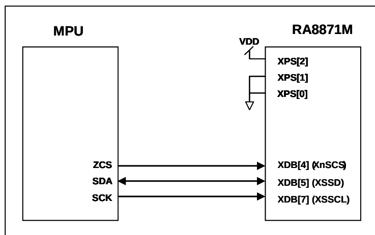
Figure 7-7 : The MPU Interface Diagram of 3-Wire SPI
