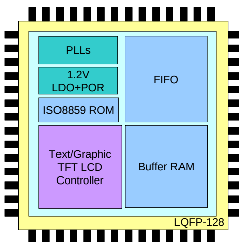
Figure 1-2 : Chip Diagram
