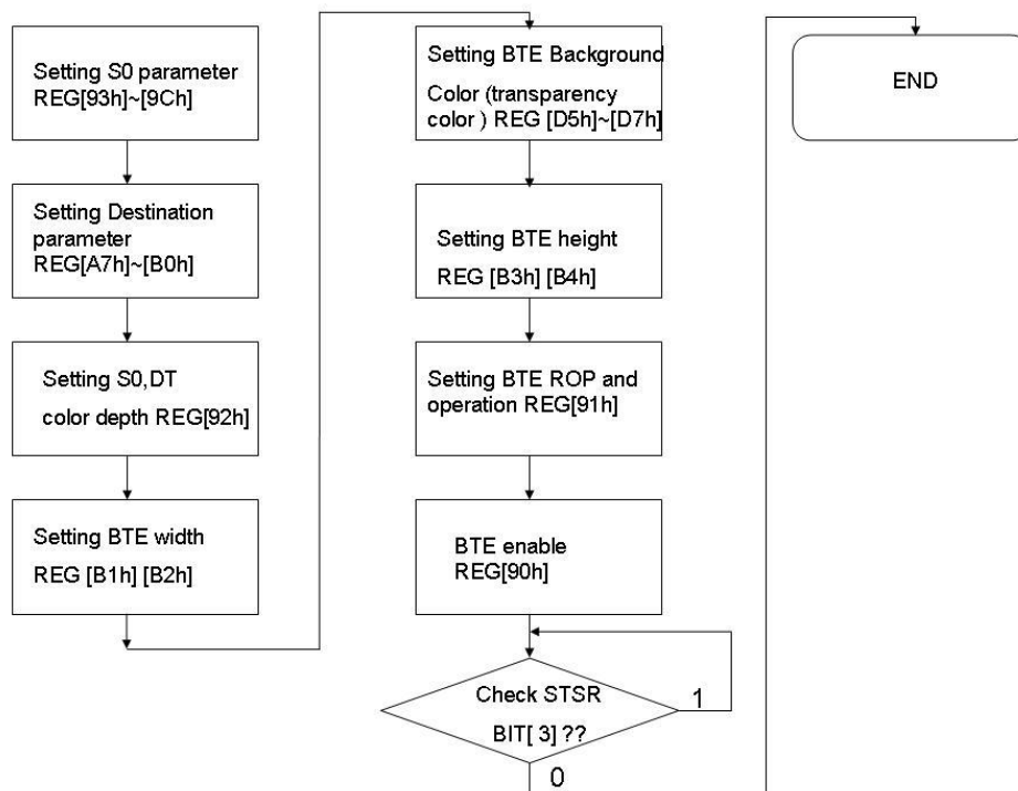
Figure 13-17 : Hardware Flow
