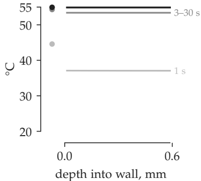
Copper 10×0.6
