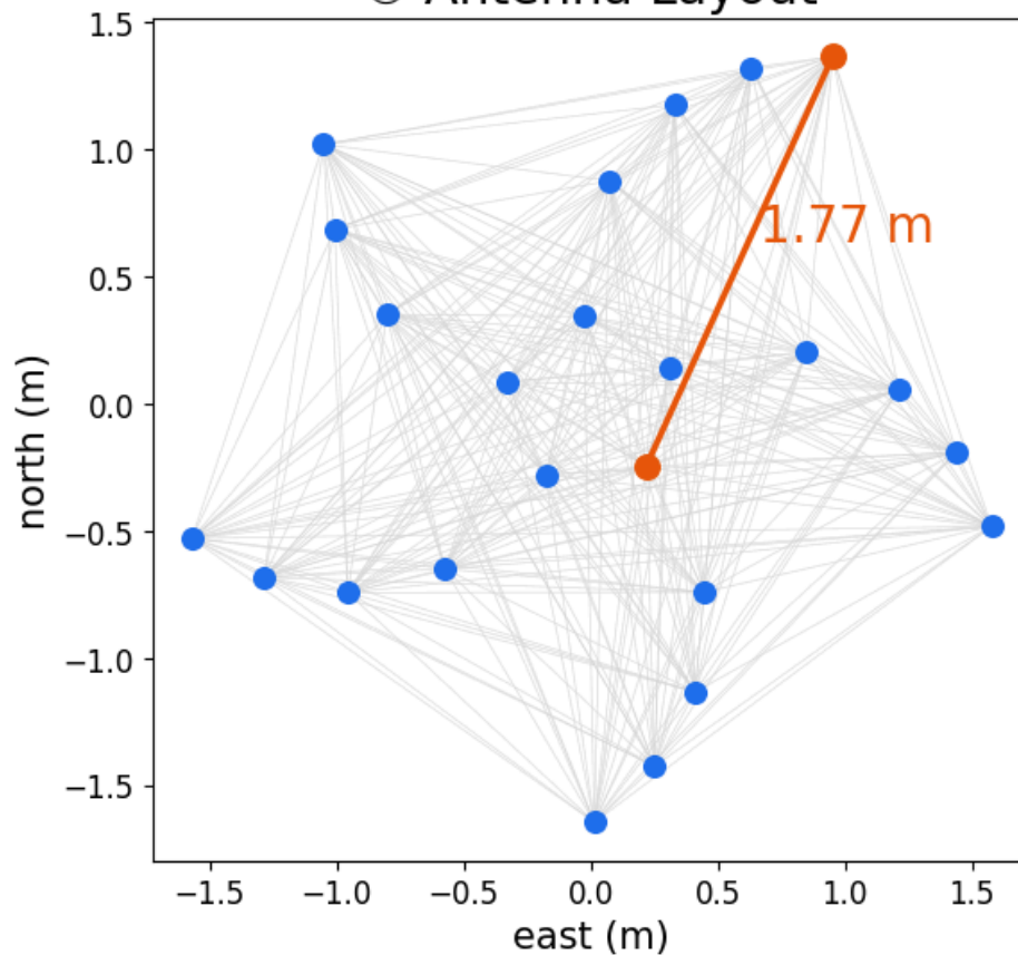
① Antenna Layout
