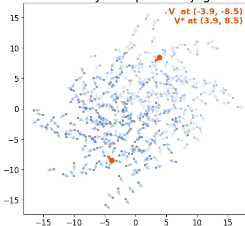
⑤ Visibility Complex Conjugates
