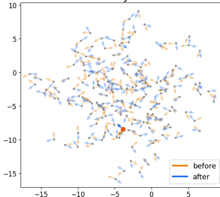
③ Visibility Vectors
