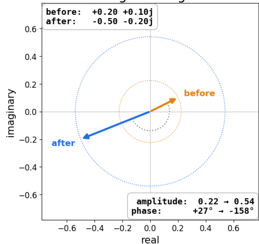
④ Argand Diagram
