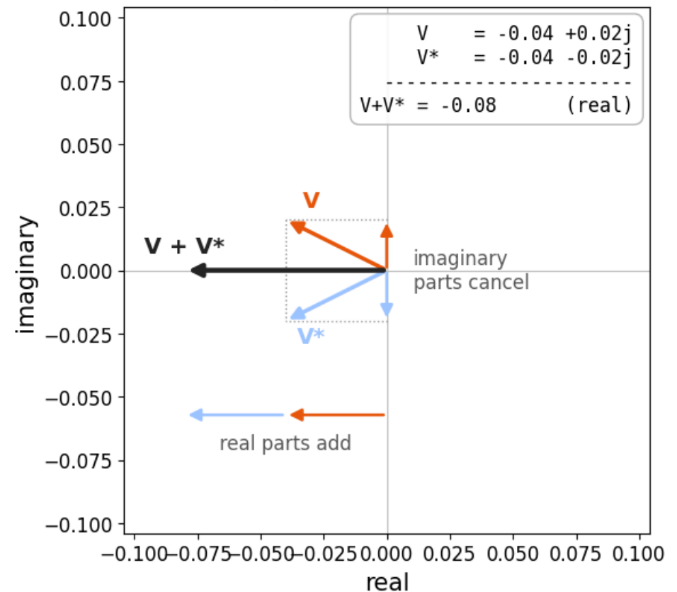
⑥ V + V^* is real
