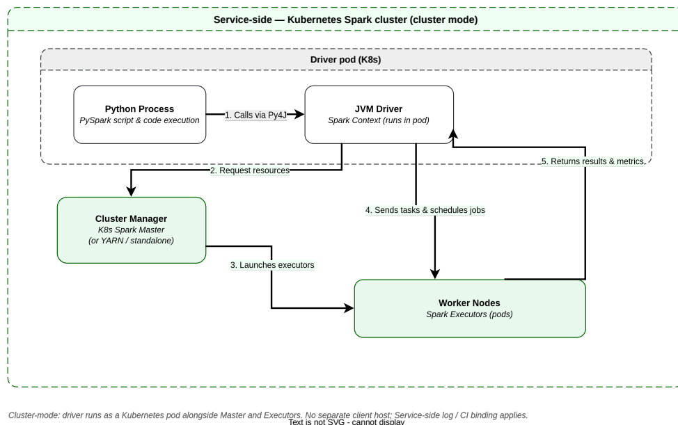
Figure 4. Spark Cluster Mode Architecture
