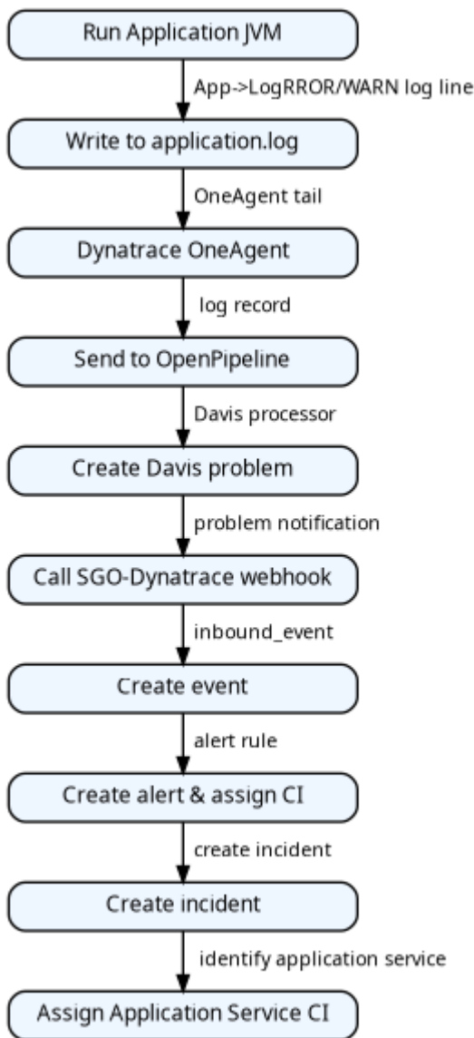
Figure 2. Log to Incident end-to-end data flow
