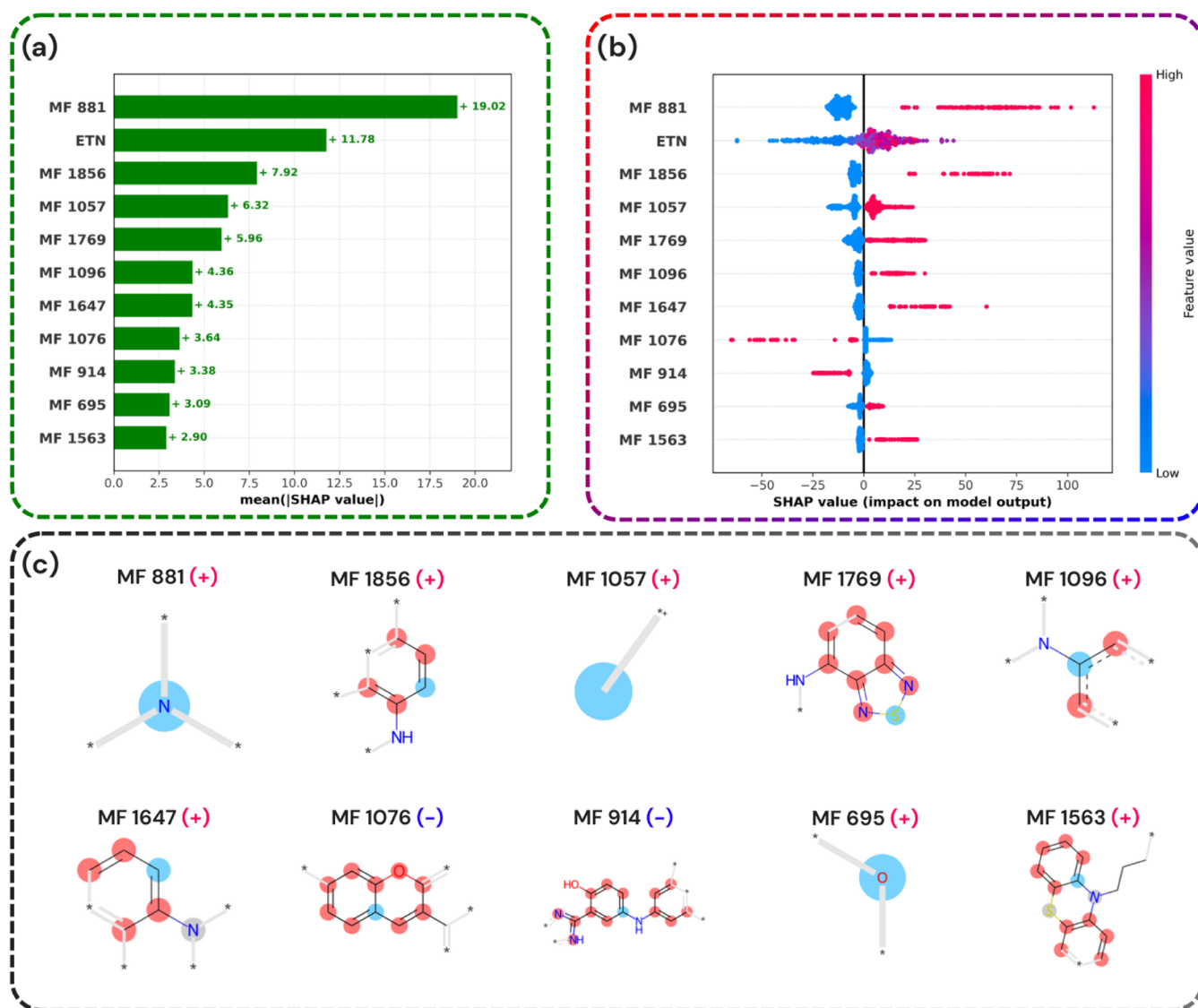
Figure 5. Visualization of SHAP analysis and molecular features influencing the predictive \lambda_{\max}^{\text{em}} model. (a) Mean SHAP values of top molecular features (MFs) highlight their overall importance. (b) Bee swarm plot showing SHAP values for each molecular feature with color indicating feature magnitude (high: red, low: blue). (c) Molecular structures of selected features, classified as positively (+) or negatively (−) contributing to the model's output.
