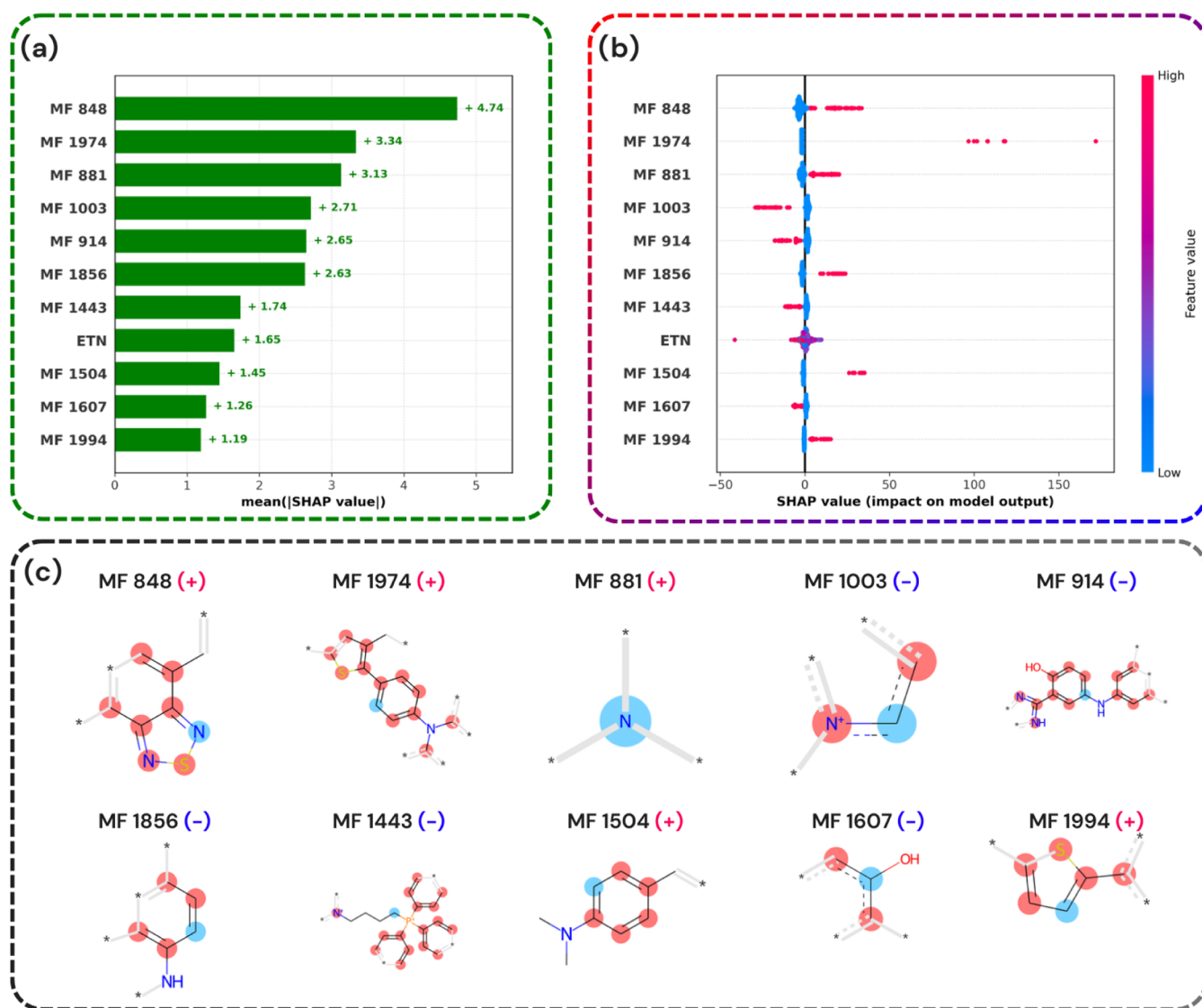
Figure 4. Visualization of SHAP analysis and molecular features influencing the predictive \lambda_{\max}^{\text{abs}} model. (a) Mean SHAP values of top molecular features (MFs) highlight their overall importance. (b) Bee swarm plot showing SHAP values for each molecular feature with color indicating feature magnitude (high: red, low: blue). (c) Molecular structures of selected features, classified as positively (+) or negatively (−) contributing to the model's output.
