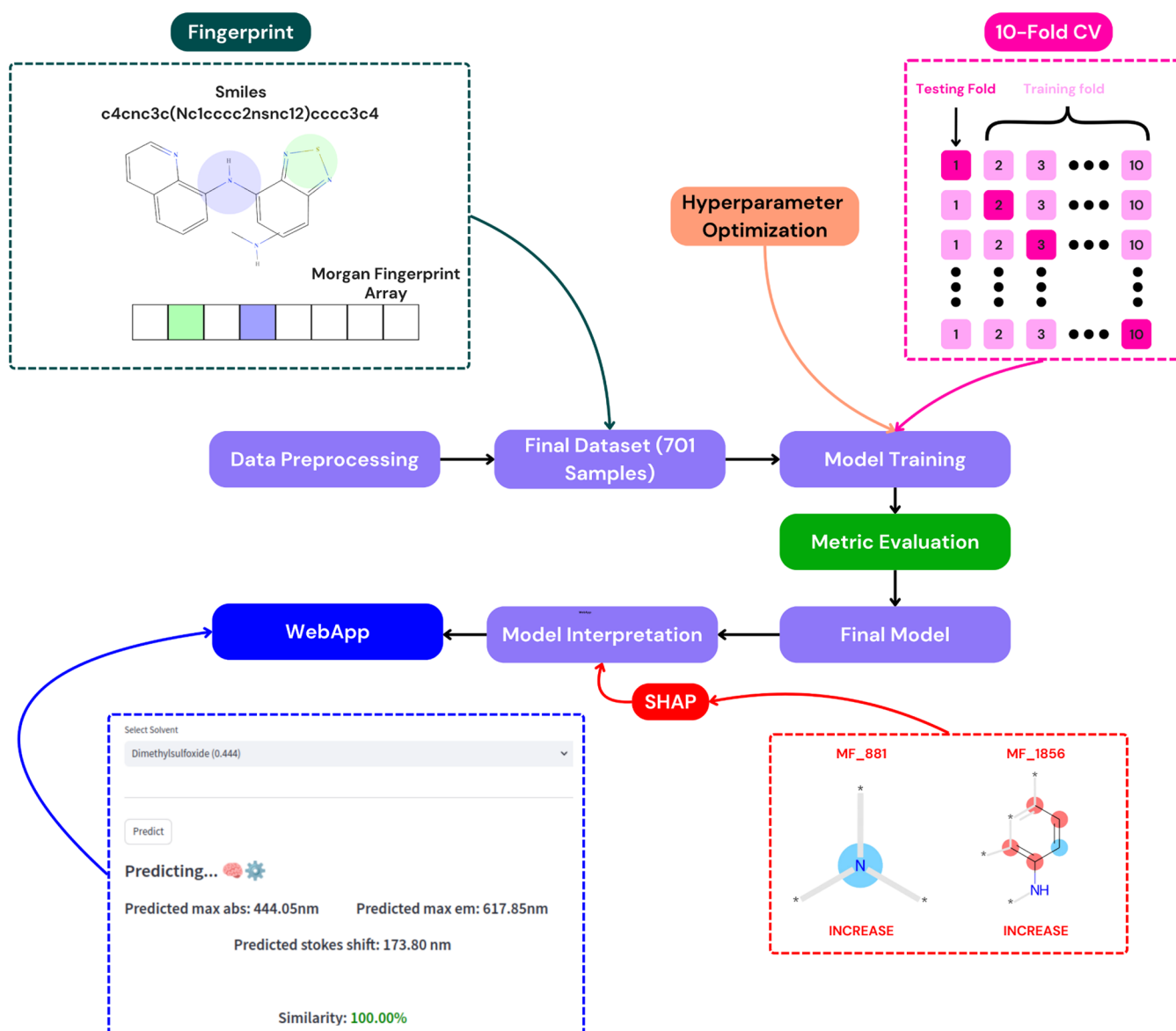
Figure 2. Schematic representation of the model development workflow, illustrating key steps, including data collection, preprocessing, fingerprint generation, hyperparameter optimization using Optuna, 10-fold cross-validation, model training with 3 algorithms (eXtreme Gradient Boosting, Random Forest, Light Gradient Boosting Machine), metric evaluation ( R^2 , Q^2 , MAE, RMSE), SHAP-based model interpretation, and deployment as a web application for prediction and visualization of results.
