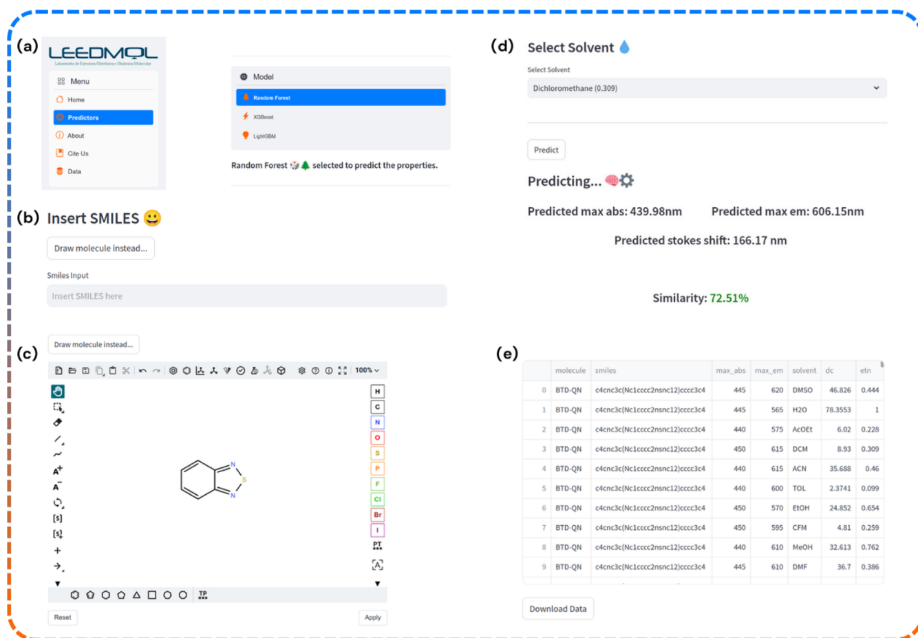
Figure 6. Overview of the WebApp workflow for predicting photophysical properties of benzothiadiazole derivatives. (a) Displays the main interface and the option to select predictive models. (b) Allows users to input SMILES or (c) draw molecular structures. (d) Presents the solvent selection and prediction results, including maximum absorption ( \lambda_{\text{max}}^{\text{abs}} ), emission ( \lambda_{\text{max}}^{\text{em}} ), Stokes shift, and structural similarity. (e) Presents the availability of the data set.
