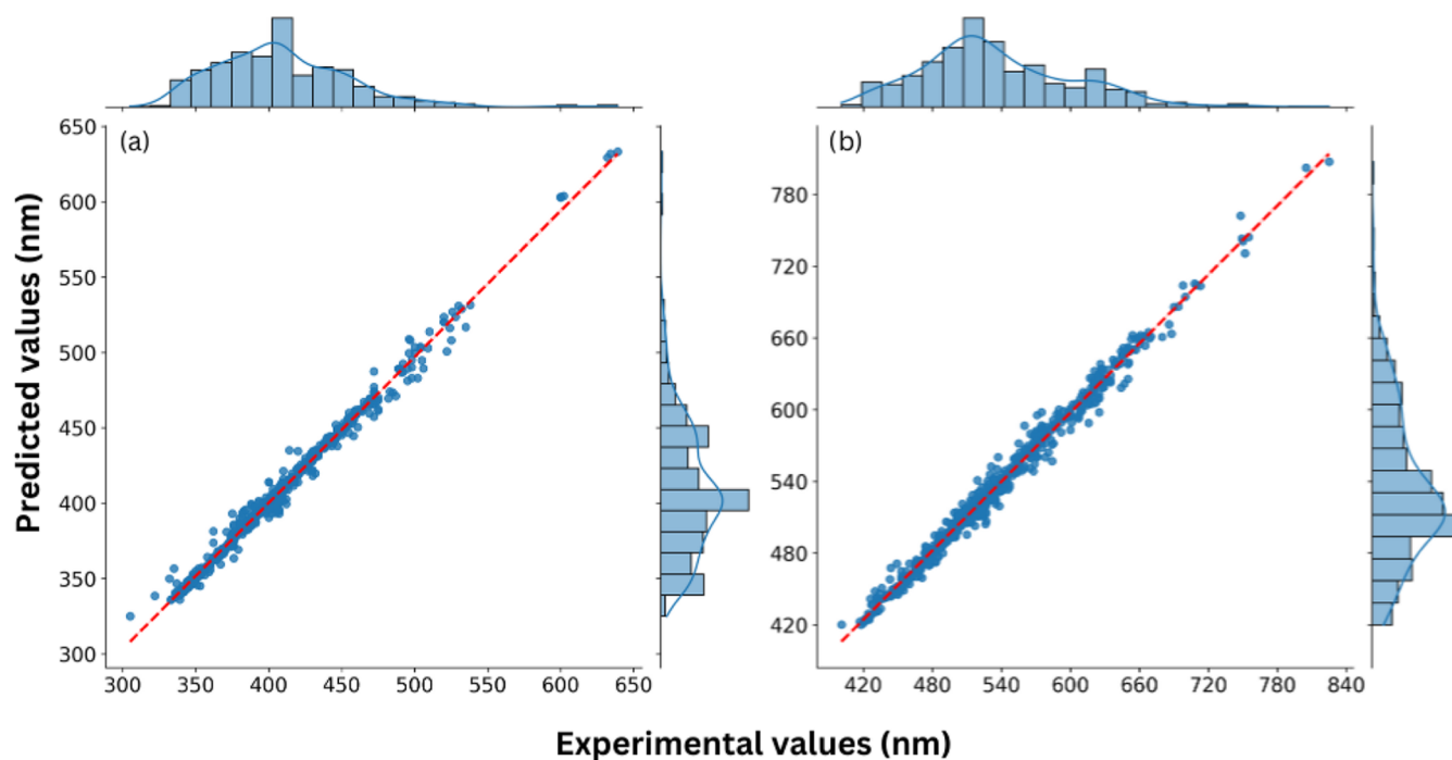
Figure 3. Predicted values versus experimental values for (a) max absorption and (b) max emission for Random Forest; red line represents the ideal prediction and blue points the actual prediction.
