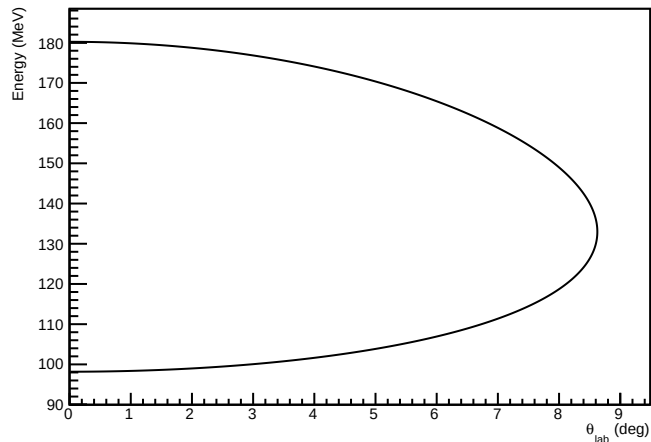
Kinematics for ^{16}\text{C}(^2\text{H}, ^3\text{H})^{15}\text{C} at 11.5 AMeV (Scatter)
