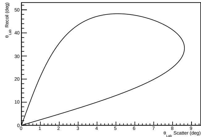
Kinematics for ^{16}\text{C}(^2\text{H}, ^3\text{H})^{15}\text{C} at 11.5 AMeV (Recoil vs Scatter)
