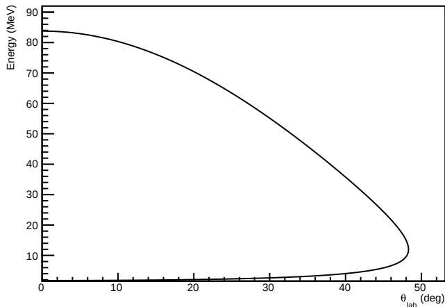
Kinematics for ^{16}\text{C}(^2\text{H}, ^3\text{H})^{15}\text{C} at 11.5 AMeV (Recoil)
