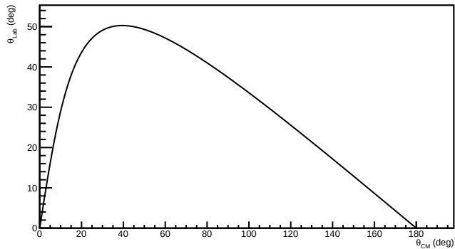
Kinematics for ^{16}\text{C}(^2\text{H},^3\text{H})^{15}\text{C} at 11.5 AMeV (Recoil)
