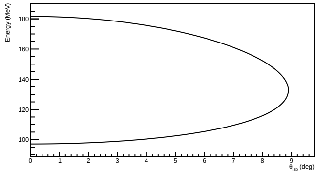
Kinematics for ^{16}\text{C}(^2\text{H},^3\text{H})^{15}\text{C} at 11.5 AMeV (Scatter)
