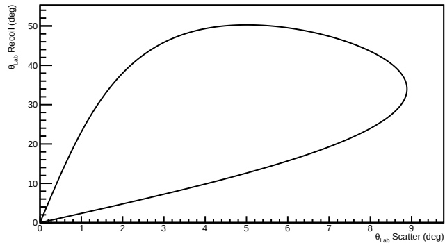
Kinematics for ^{16}\text{C}(^2\text{H},^3\text{H})^{15}\text{C} at 11.5 AMeV (Recoil vs Scatter)
