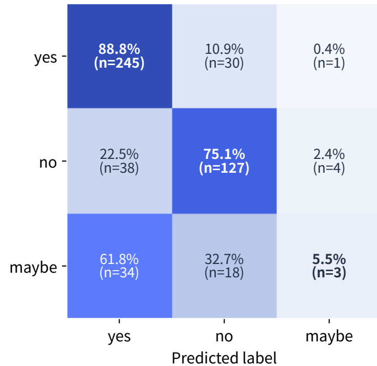
Full
