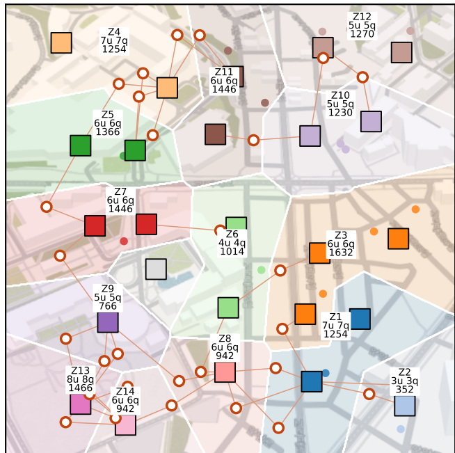
(a) partition under a 2000 two-qubit budget 25 APs, 50 UEs \rightarrow 14 zones, |\mathcal{B}|=30 boundary UEs (60%)
