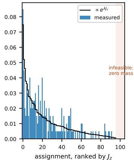
(b2) zone Z1: 4 APs, N_z=7 , |\mathcal{F}_z|=96
