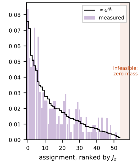
(b4) zone Z10: 2 APs, N_z=7 , |\mathcal{F}_z|=54
