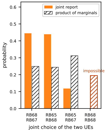
(c1) zone Z3, boundary UEs 0 & 18
