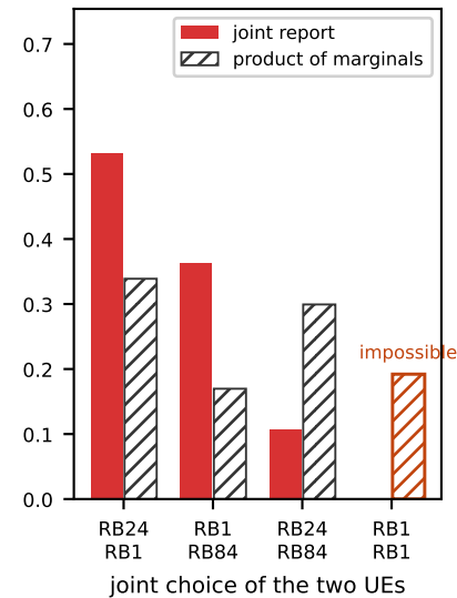
(c2) zone Z7, boundary UEs 1 & 37
