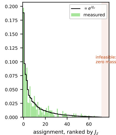
(b3) zone Z6: 2 APs, N_z=7 , |\mathcal{F}_z|=72
