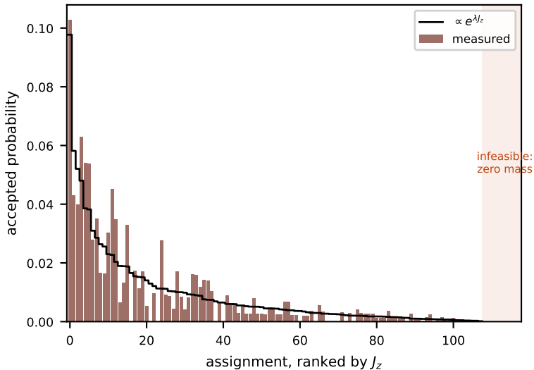
(b1) zone Z11: 1 AP, N_z=9 , |\mathcal{F}_z|=108
