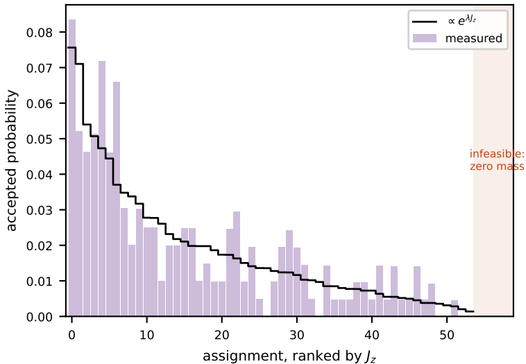
(b4) zone Z10: 2 APs, N_z=7 , |\mathcal{F}_z|=54
