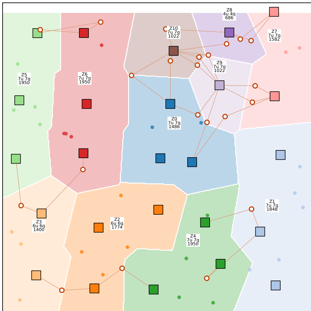
(a) partition under a 2000 two-qubit budget 25 APs, 50 UEs \rightarrow 11 zones, |\beta|=22 boundary UEs (44%)
