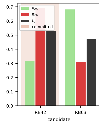
boundary UE 40: Z5 + Z6 confidence 0.53
