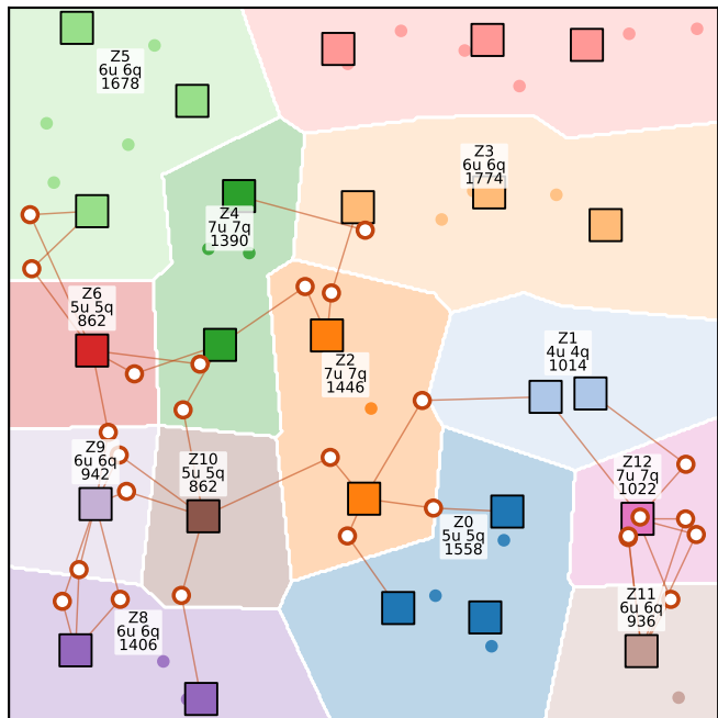
(a) partition under a 2000 two-qubit budget 25 APs, 50 UEs \rightarrow 13 zones, |\mathcal{B}|=26 boundary UEs (52%)
