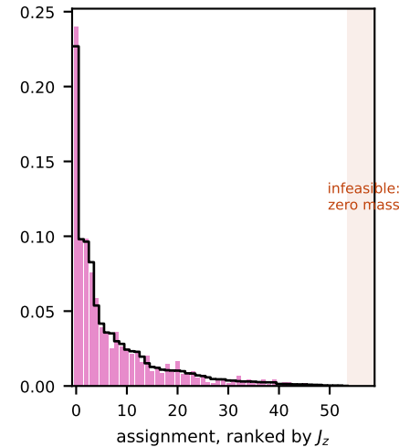
zone Z12: N_z=7 , |\mathcal{F}_z|=54 \mu_z=0.001 , k=26 rounds
