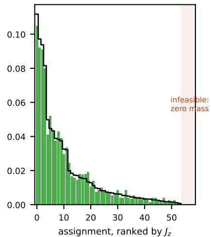
zone Z4: N_z=7 , |\mathcal{F}_z|=54 \mu_z=0.015 , k=6 rounds
