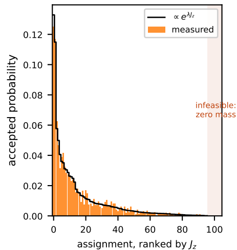
zone Z2: N_z=7 , |\mathcal{F}_z|=96 \mu_z=0.026 , k=4 rounds
