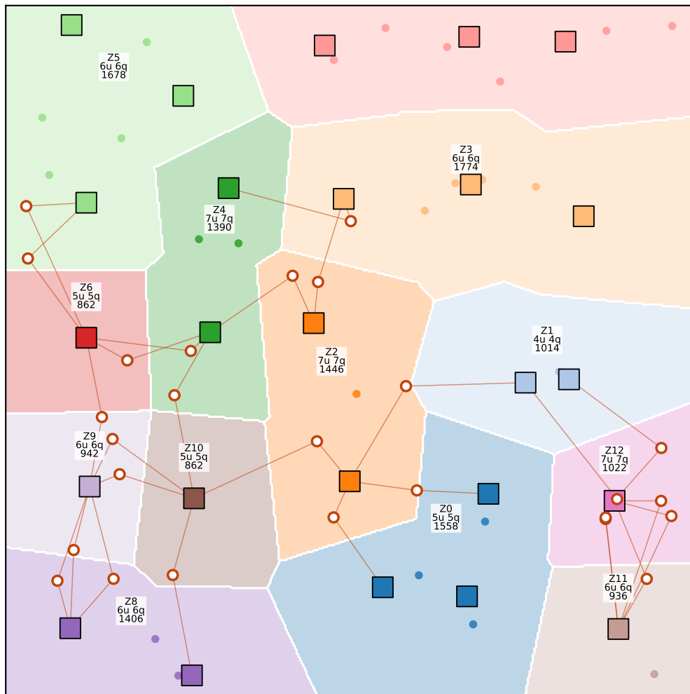
(a) partition under a 2000 two-qubit budget 25 APs, 50 UEs → 13 zones, |\beta|=26 boundary UEs (52%)
