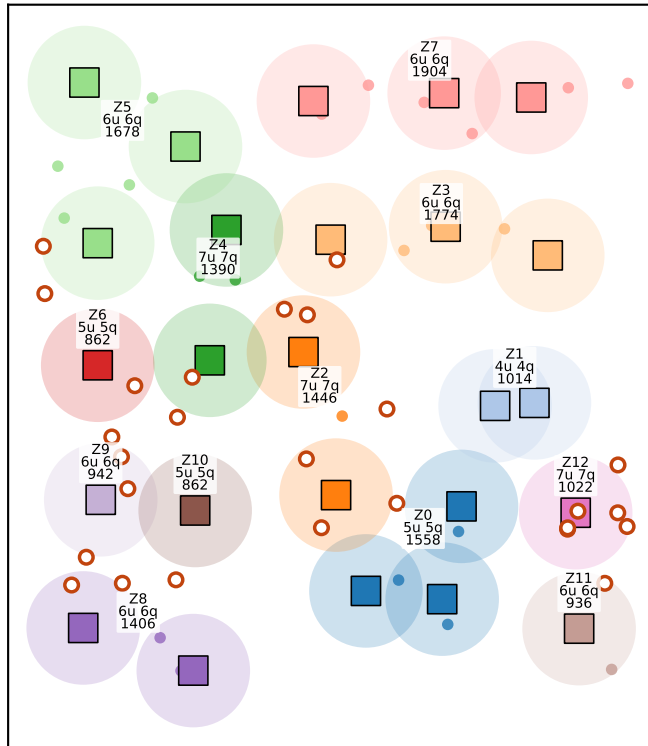
(a) partition under a 2000 two-qubit budget 25 APs, 50 UEs \rightarrow 13 zones, |B|=26 boundary UEs (52%)
