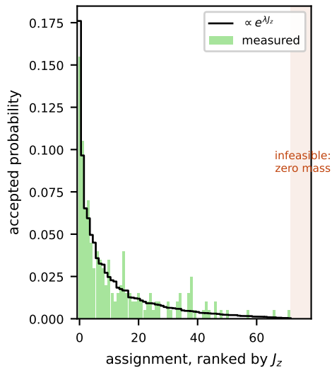
(b1) zone Z5: 2 APs, N_z=7 , |\mathcal{F}_z|=72
