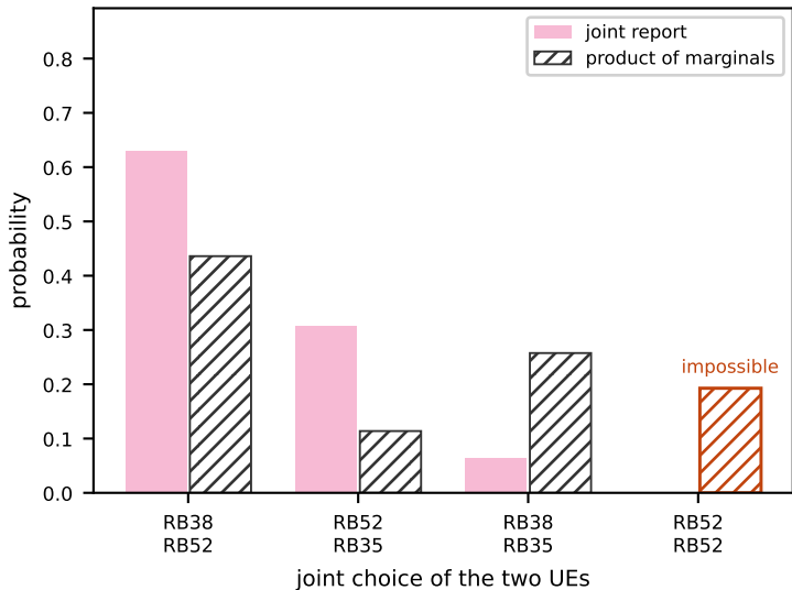
(c1) zone Z13, boundary UEs 12 & 14
