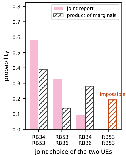
(c1) zone Z13, boundary UEs 6 & 16
