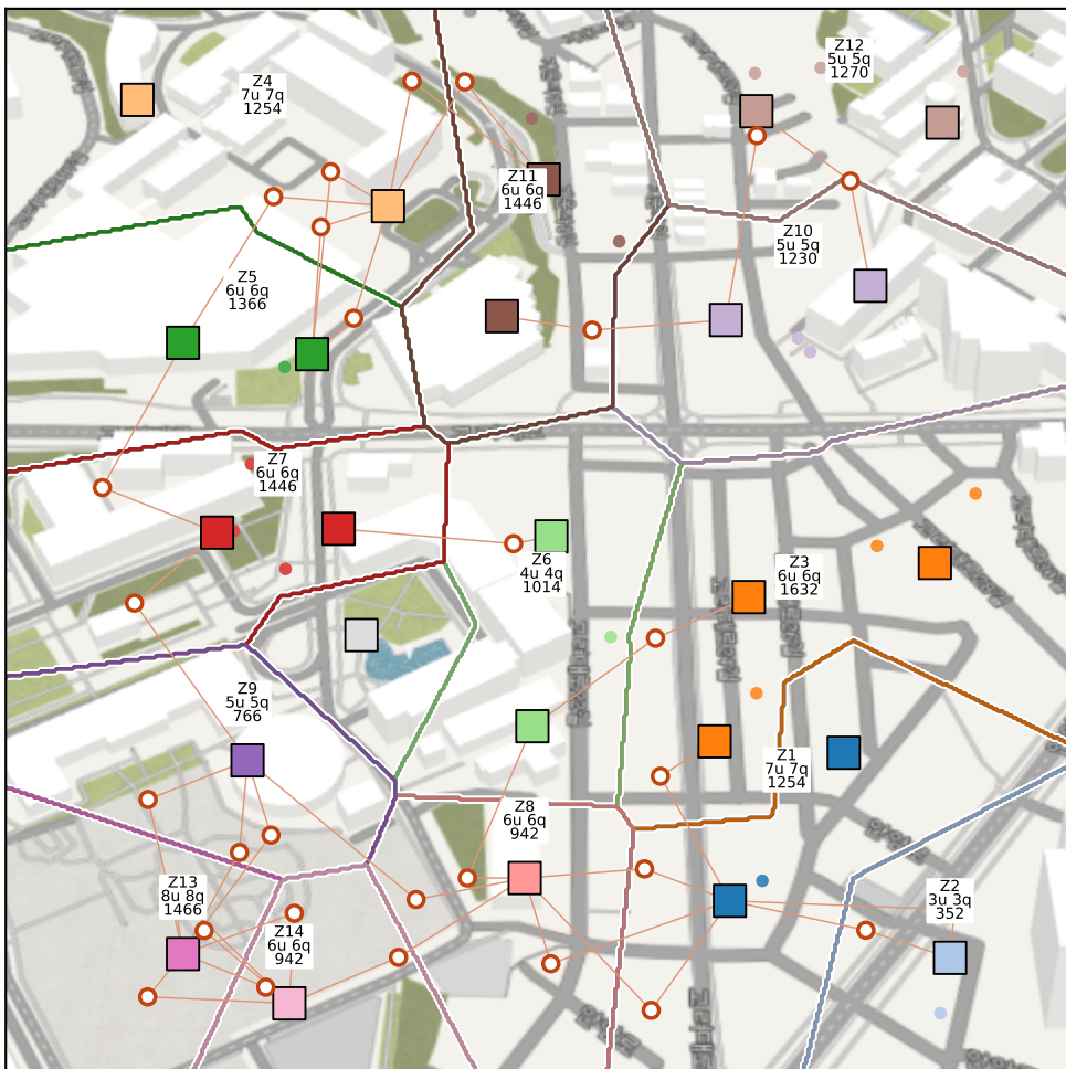
(a) partition under a 2000 two-qubit budget 25 APs, 50 UEs → 14 zones, |\beta|=30 boundary UEs (60%)
