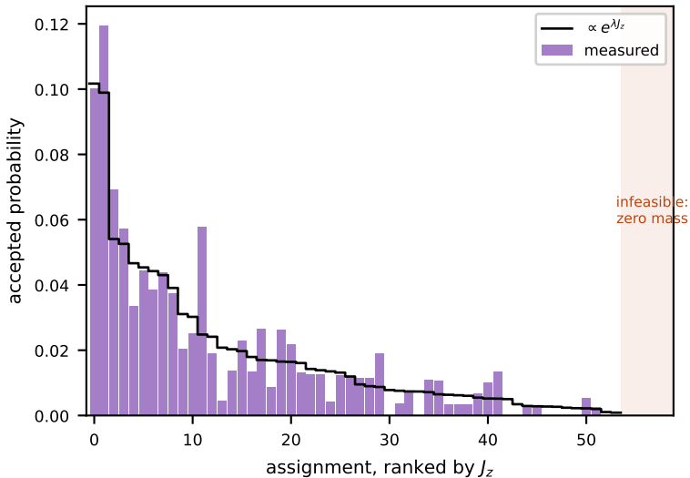
(b2) zone Z8: 2 APs, N_z=7 , |\mathcal{F}_z|=54
