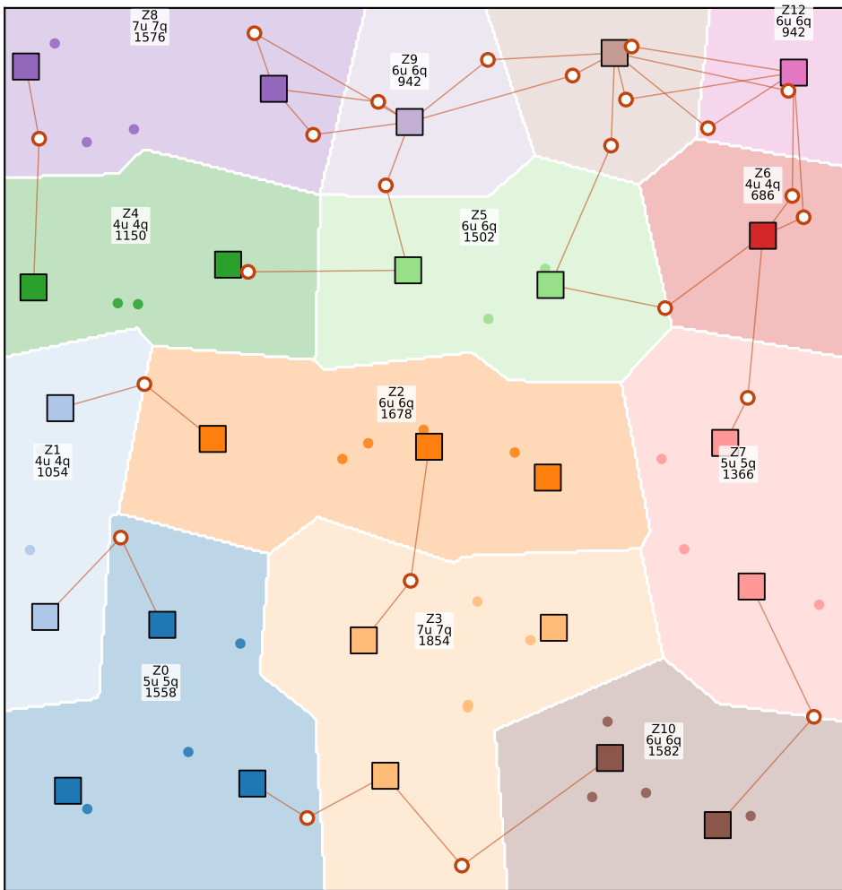
(a) partition under a 2000 two-qubit budget 25 APs, 50 UEs \rightarrow 13 zones, |\beta|=23 boundary UEs (46%)
