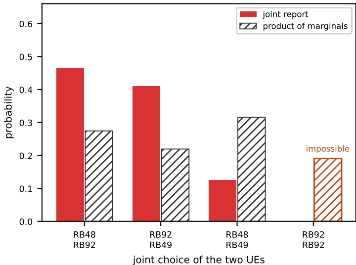
(c2) zone Z6, boundary UEs 25 & 39
