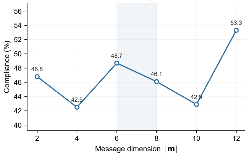
COLREGs compliance
