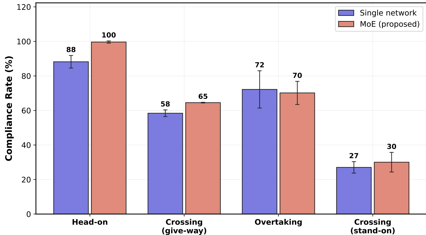
COLREGs Compliance by Encounter Situation (16 vessels)
