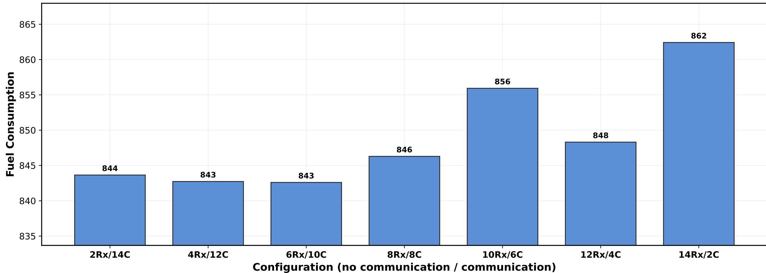
Fuel Consumption (16 vessels)
