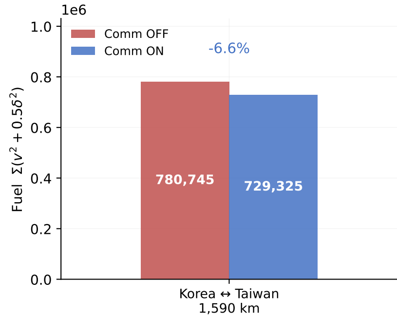
(a) Fuel per voyage
