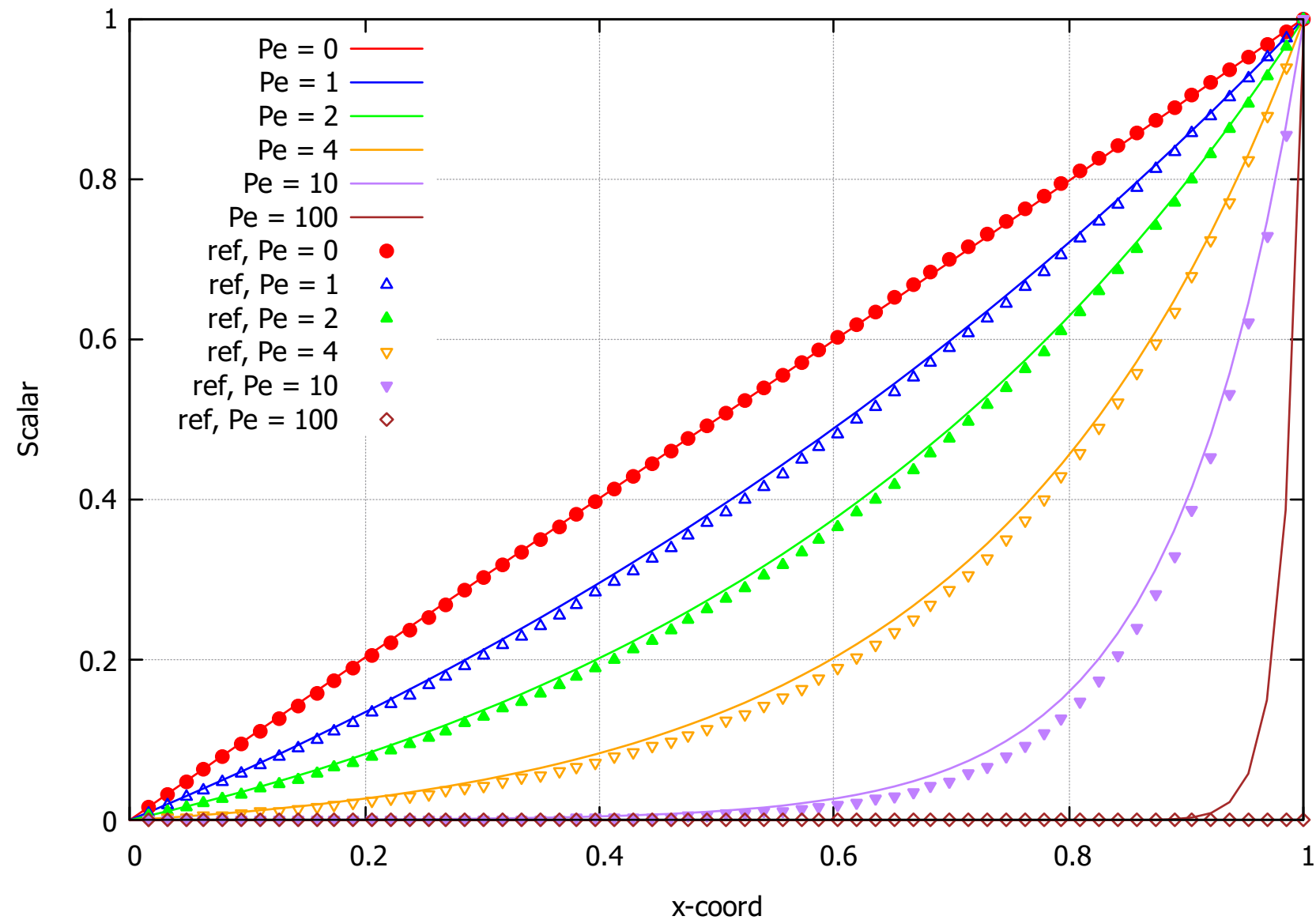
1D Convection-Diffusion along x direction
