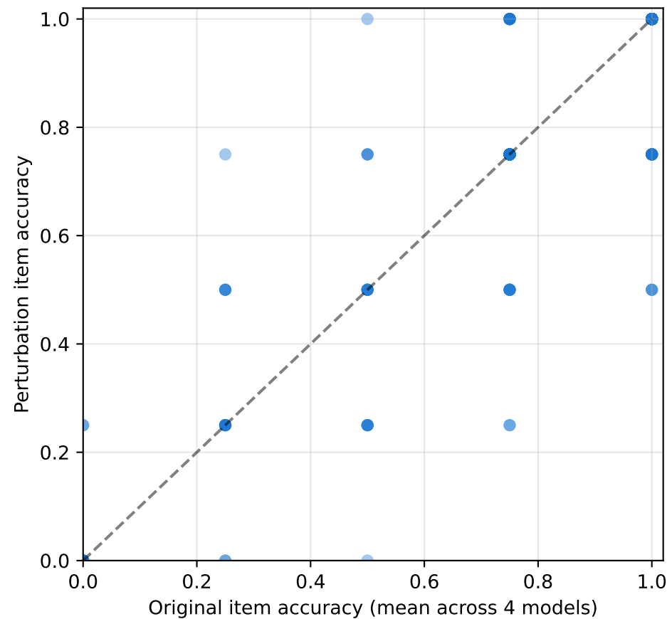
MMLU r = 0.878 , shift = +0.016
