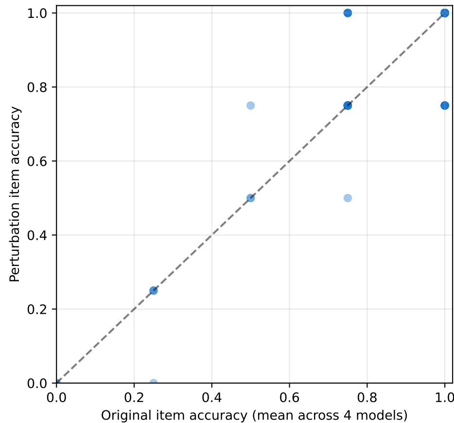
ARC r = 0.890 , shift = +0.008
