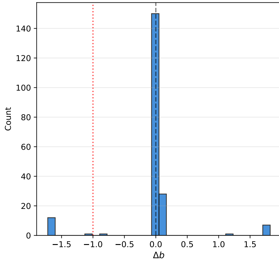
ARC-C — 6.5% items with \Delta b < -1
