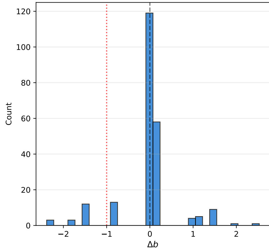
MMLU — 7.9% items with \Delta b < -1
