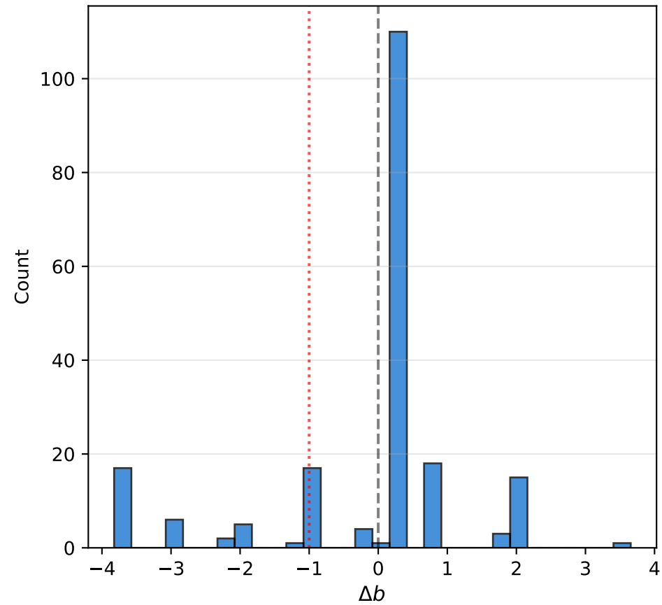
GSM8K — 23.0% items with \Delta b < -1
