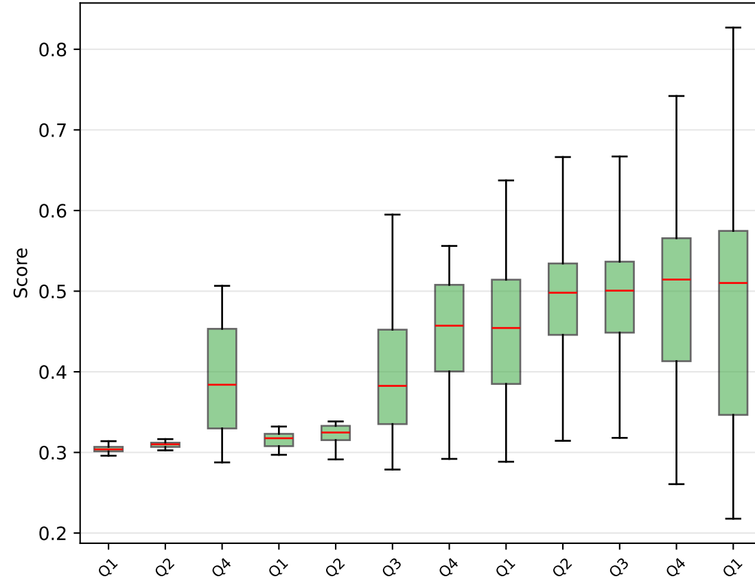
IFEval
