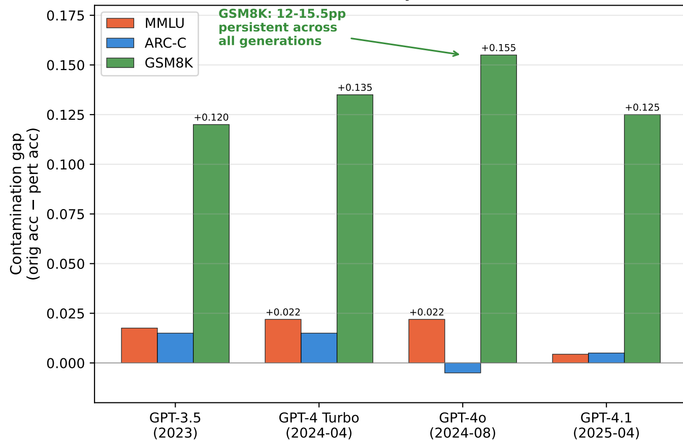
Per-Model Contamination Gap (full data, n=628 items)
