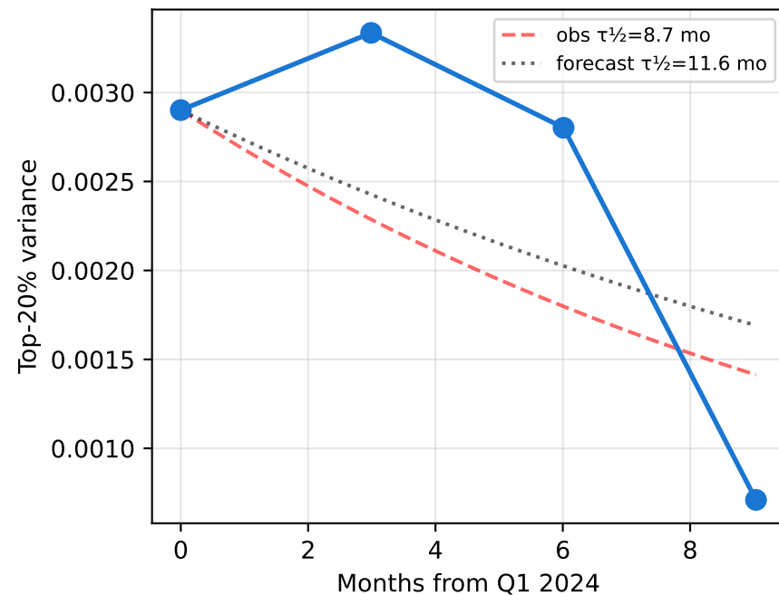
IFEval
