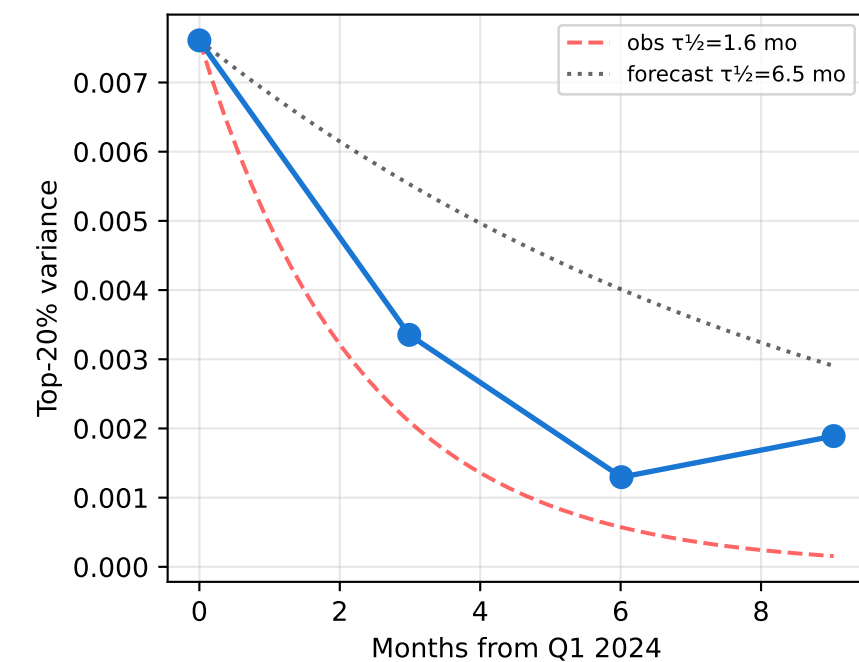
IFEval
