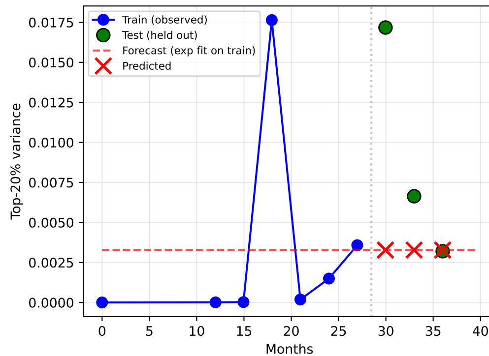
MATH_LVL5 MAPE=44.6%
