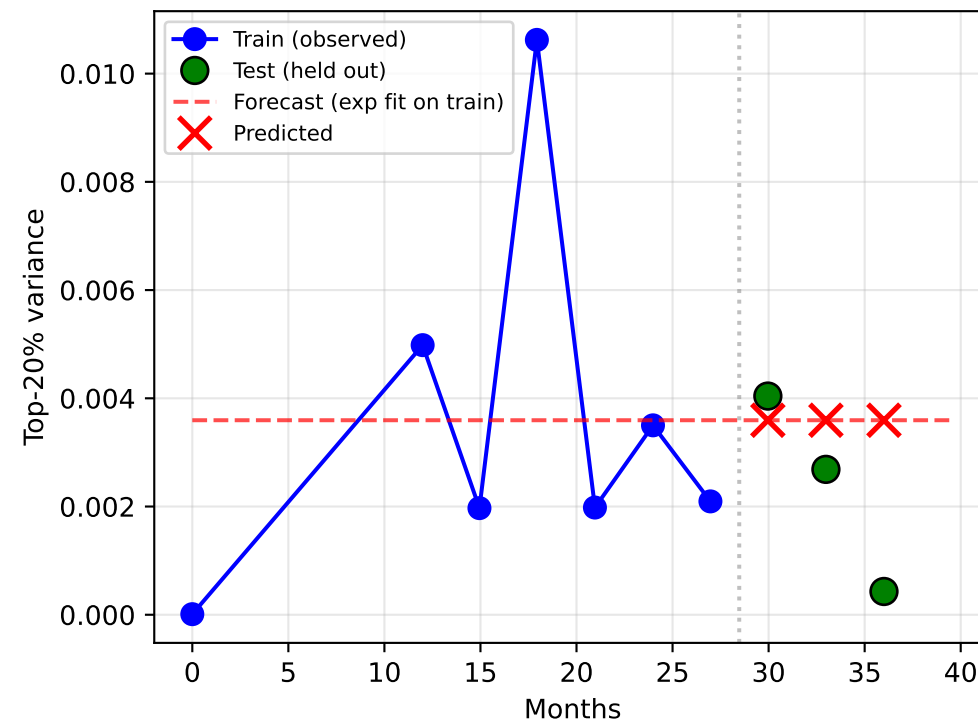
MATH_LVL5 MAPE=44.6%
