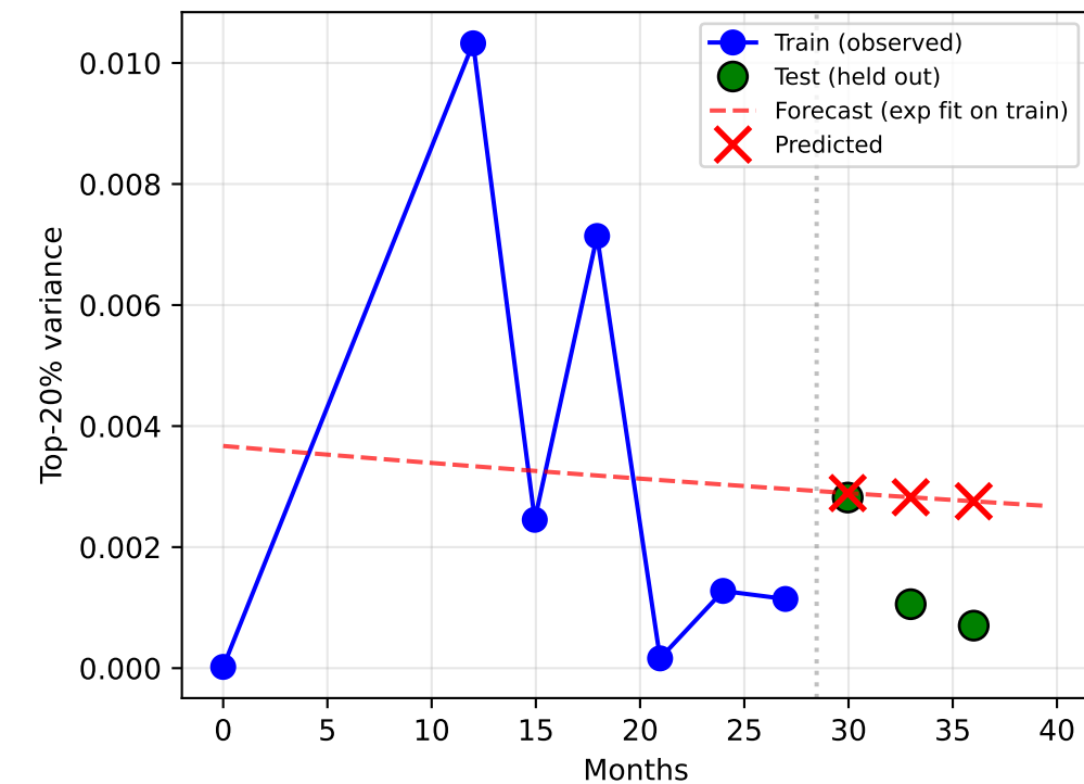
IFEVAL MAPE=136.9%
