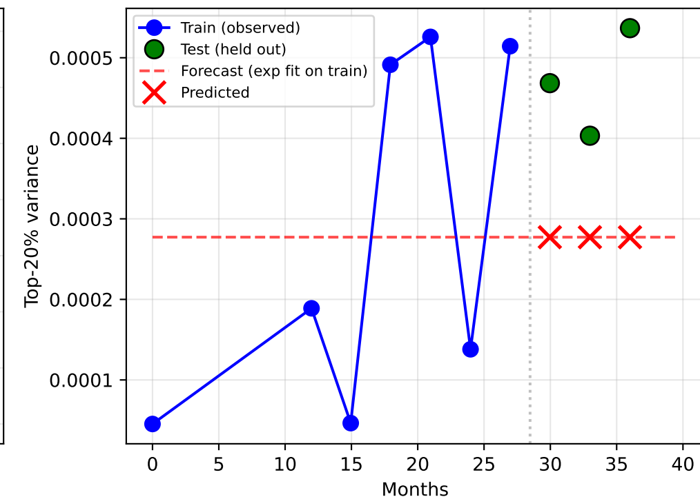
MUSR MAPE=40.1%
