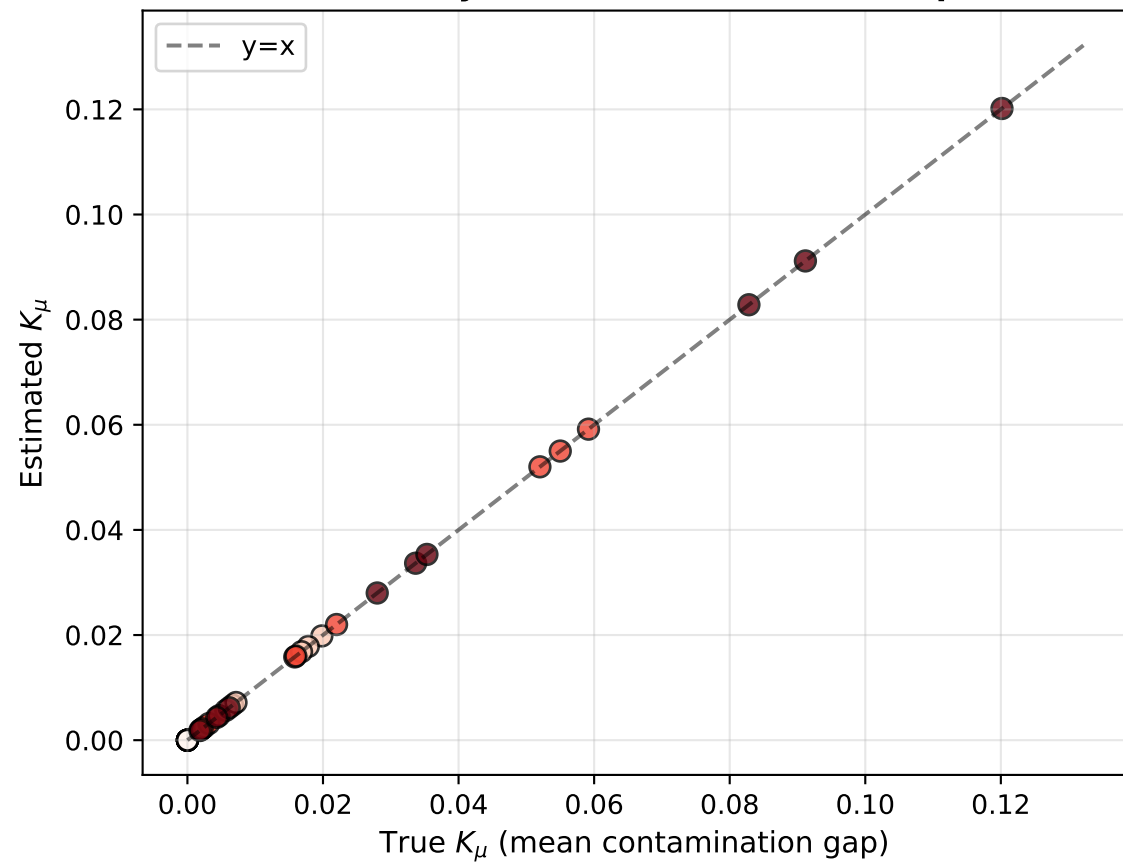
Recovery: Mean Contamination Gap
