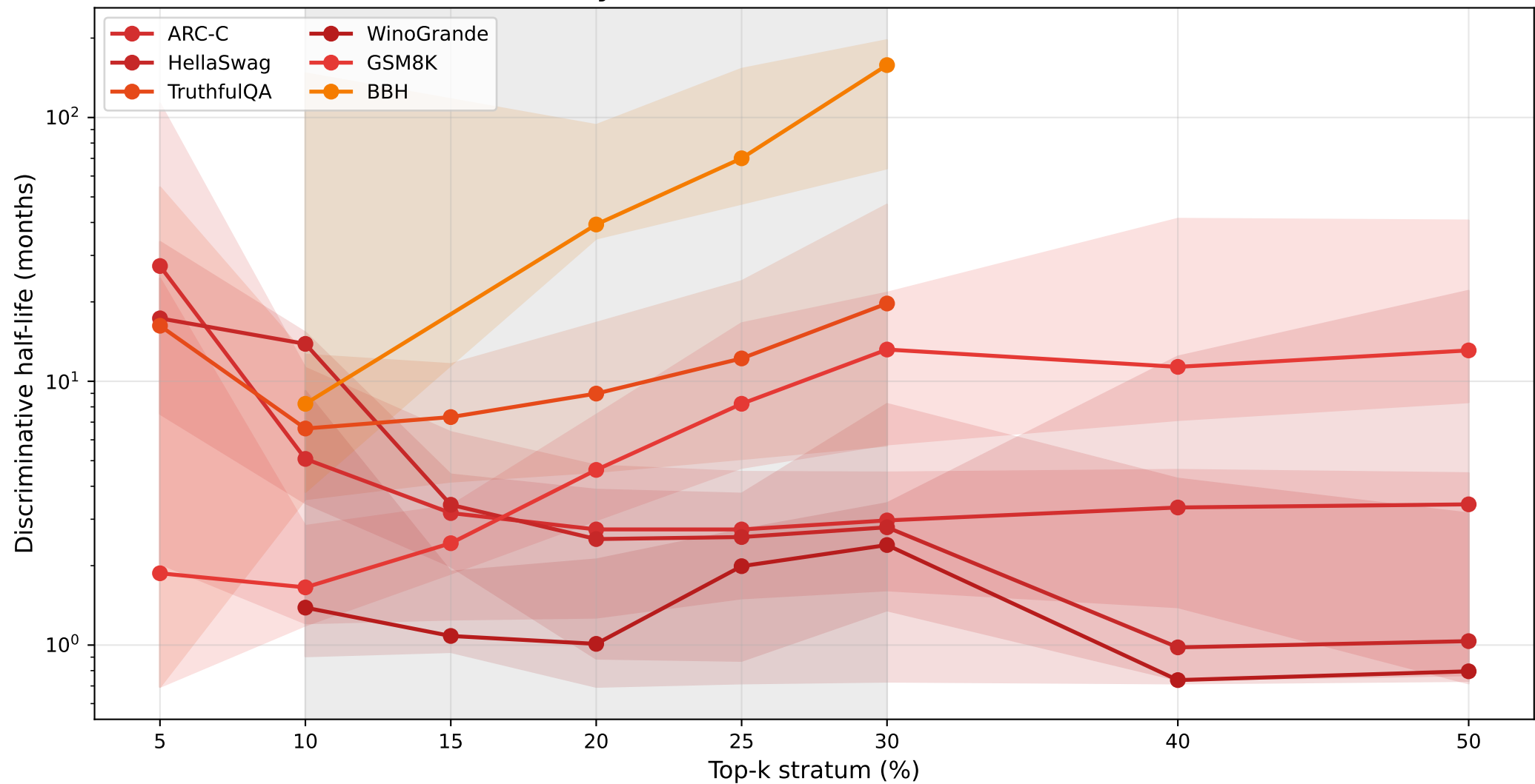
Sensitivity of Half-Life Estimates to Stratum Size
