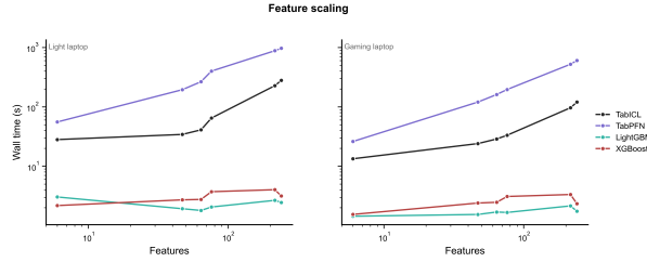
Figure 8: Feature Scale Loglog Time
