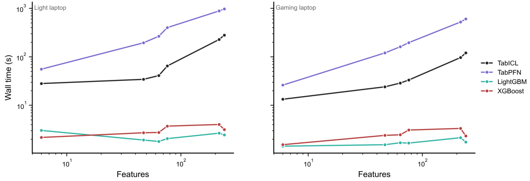
Figure 5: Feature Scale Loglog Time
