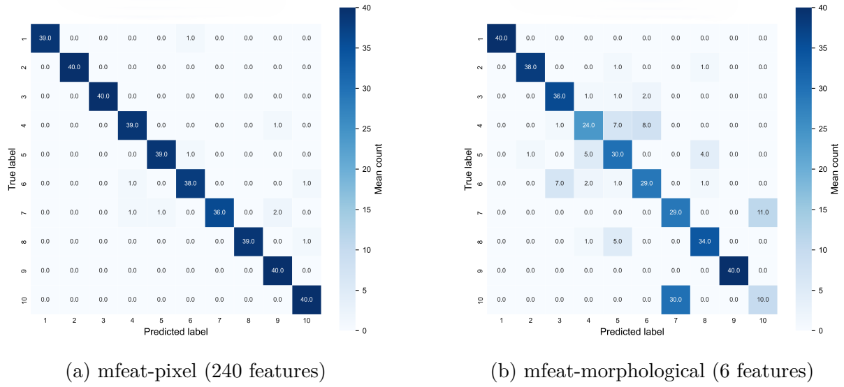
Figure 8: Confusion Matrixes of TabICL
