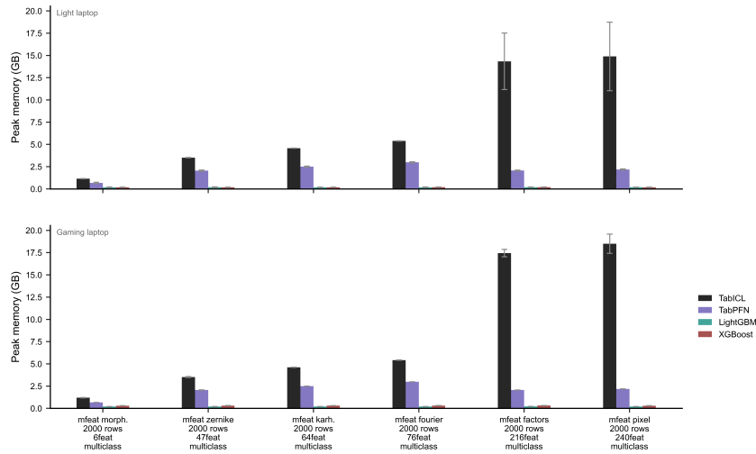
Figure 6: Feature Scale Peak-Memory Bar by Device
