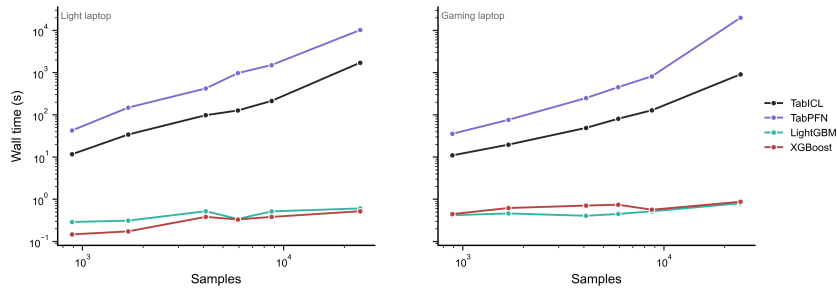
Figure 2: Time Cost Sample Scaling
