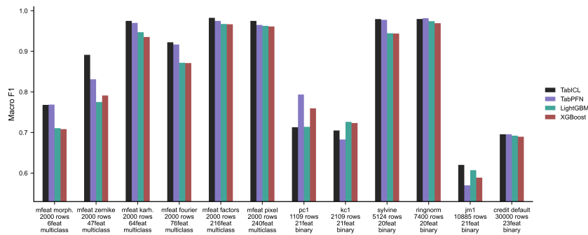
Figure 1: Performance by Dataset
