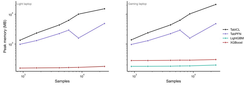
Figure 4: Memory Sample Scaling
