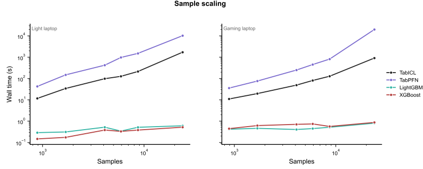
Figure 3: Time Cost Sample Scaling
