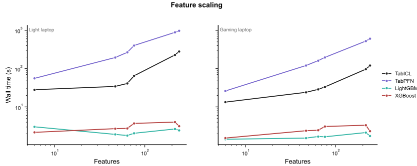
Figure 7: Feature Scale Loglog Time
