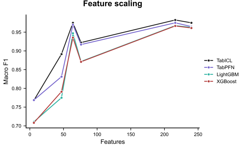
Figure 6: Feature Macro-F1 Scaling
