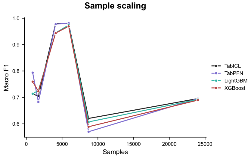
Figure 2: Macro-F1 Sample Scaling
