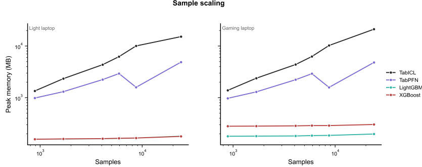
Figure 5: Memory Sample Scaling
