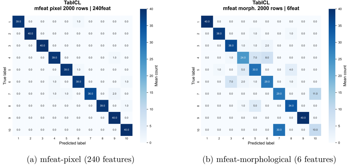
Figure 10: Confusion Matrixes of TabICL
