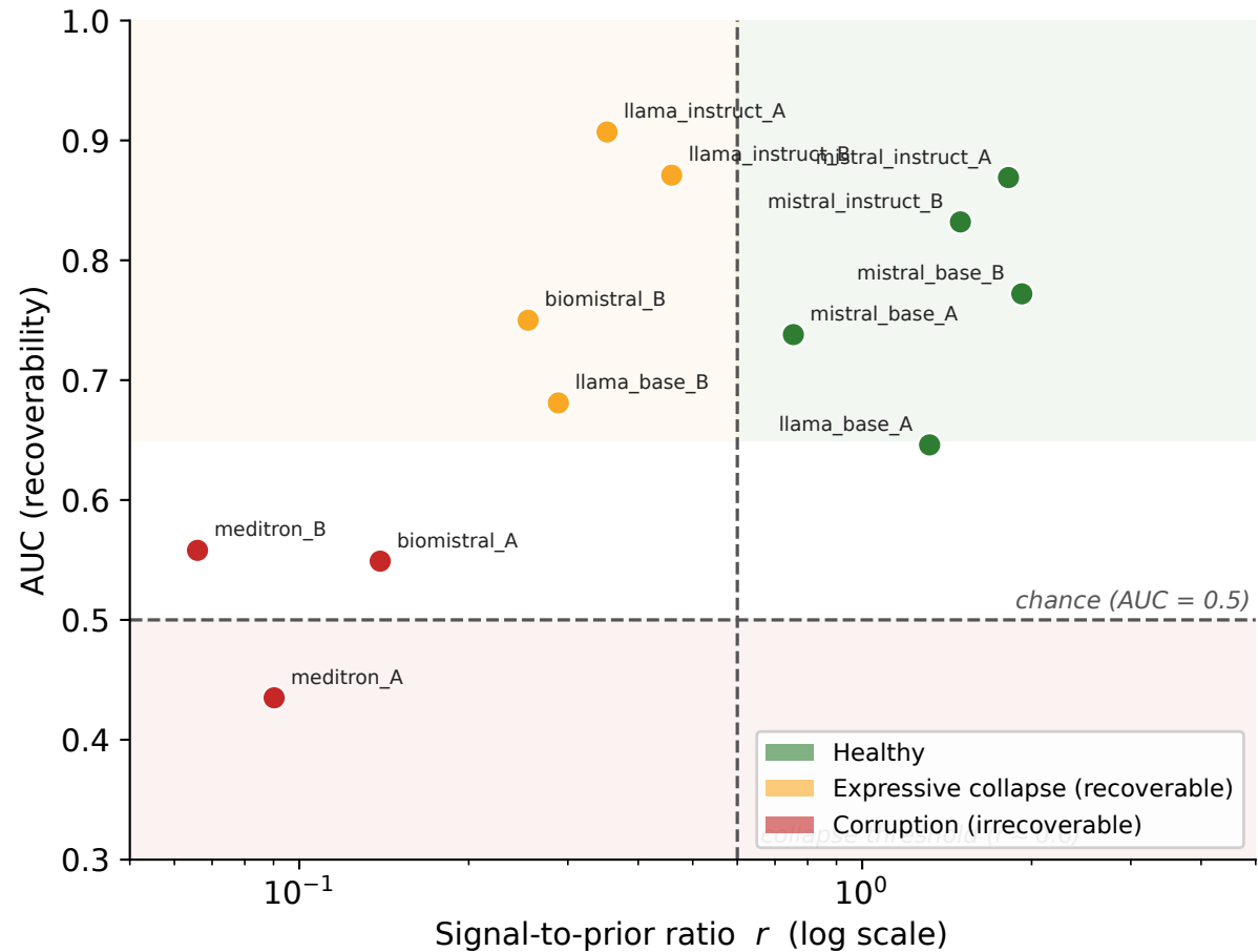
Two-dimensional mode-collapse diagnostic
