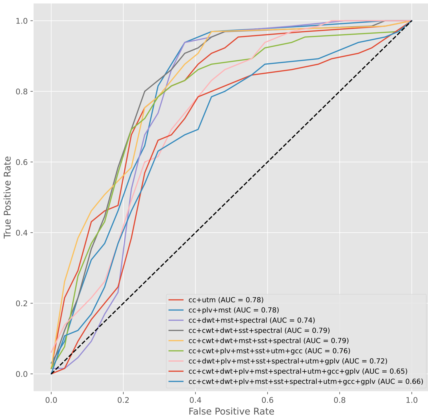
ROC Curve of ensembles
