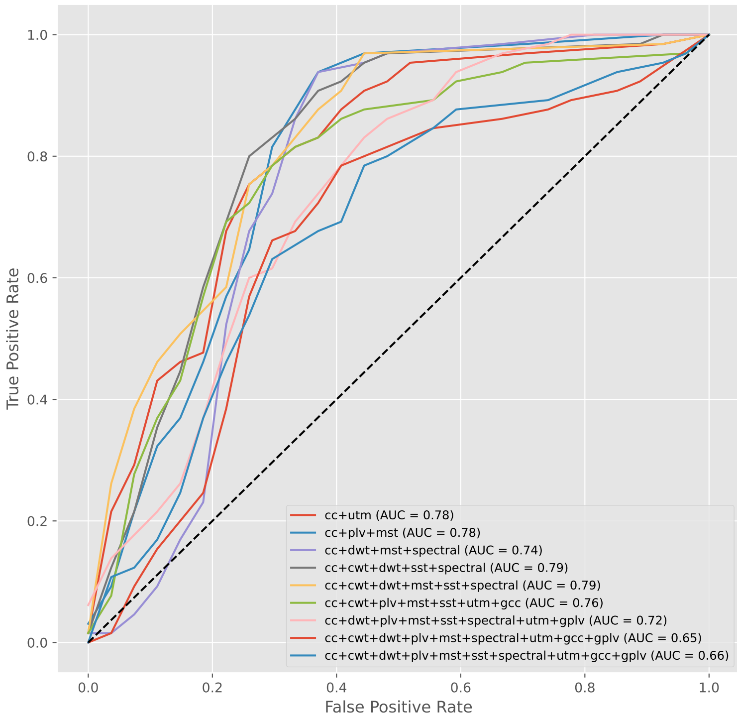
ROC Curves for Best Feature Combinations
