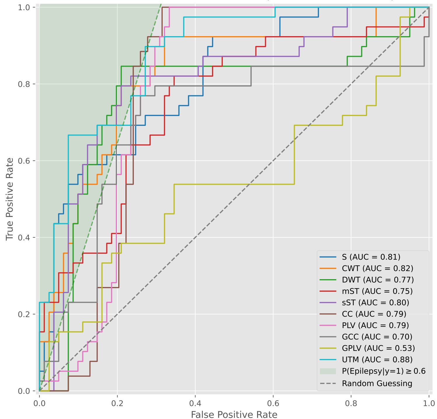
ROC Curves for Best Feature Sets (Whole Data with IEDs)
