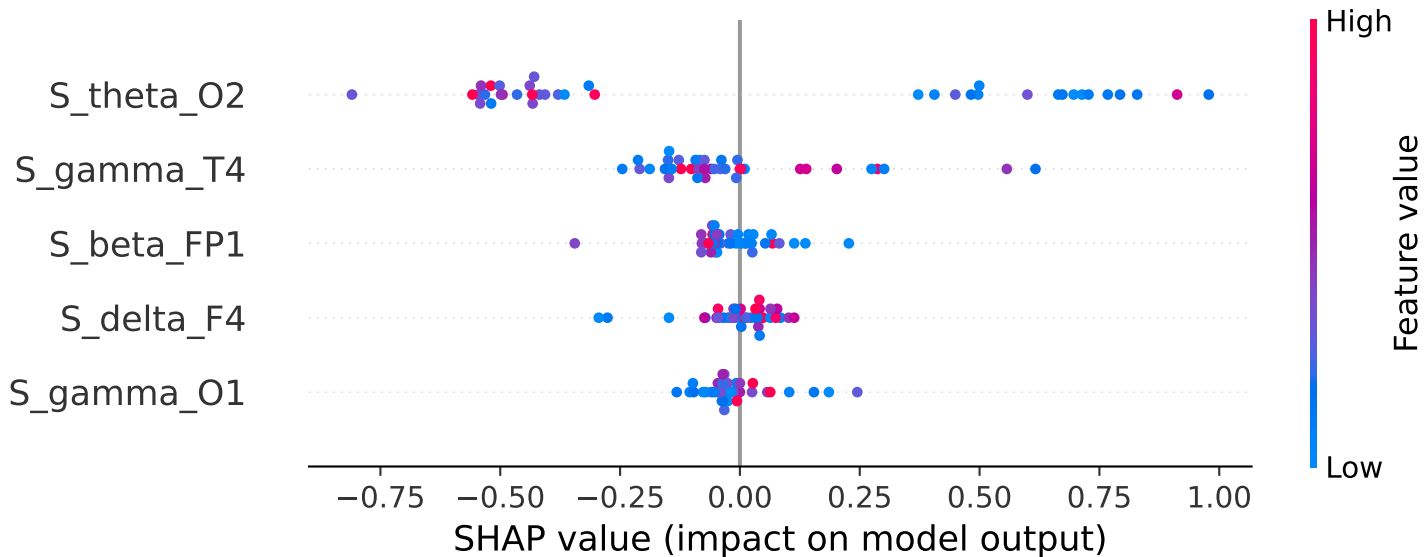
SHAP Summary Plot for spectral - montage: CAR, segment_length: 20, combiner: std
