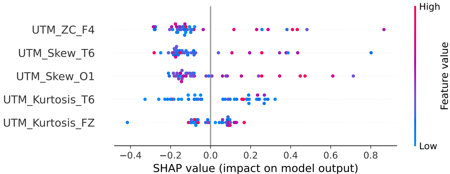
SHAP Summary Plot for utm - montage: Laplacian, segment_length: 60, combiner: mean
