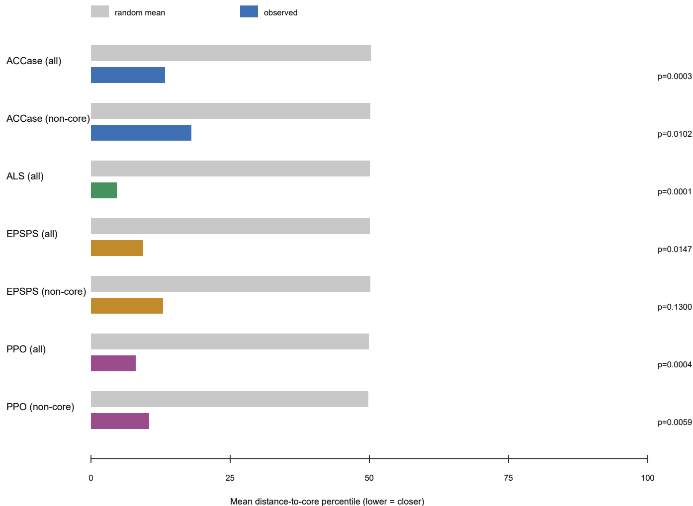
Figure 2. Observed TSR positions are enriched near active-site cores
